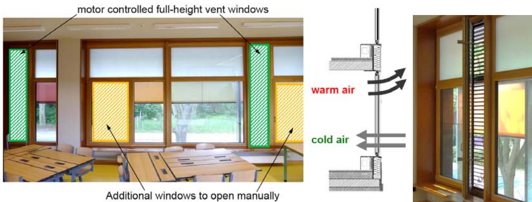
Fig. 5 Windows for natural ventilation
