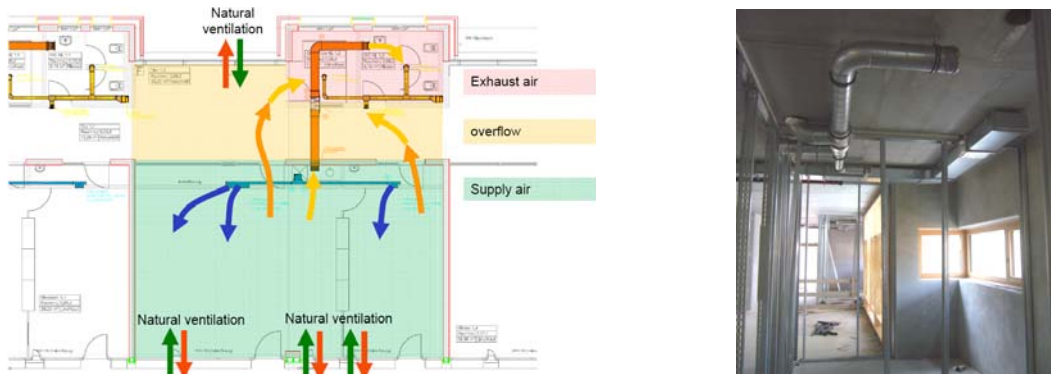
Fig. 5 Hybride ventilation scheme, simple and cheap installations
