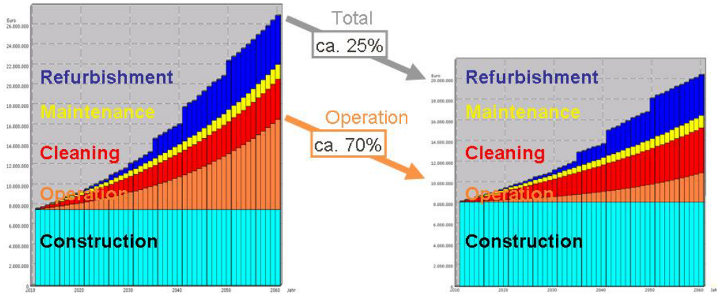
Fig. 12 Life Cycle Cost comparison of german standard new building EnEV 2009 and the new school cumulative 50 years period, mounting rate energy cots 4% per year
