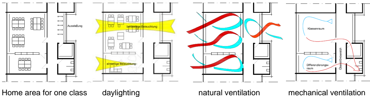
Fig. 4 Utilization and technical concept for a “home area”
