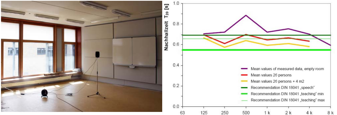
Fig.9 Interior view of a classroom, measurements of reverberation
